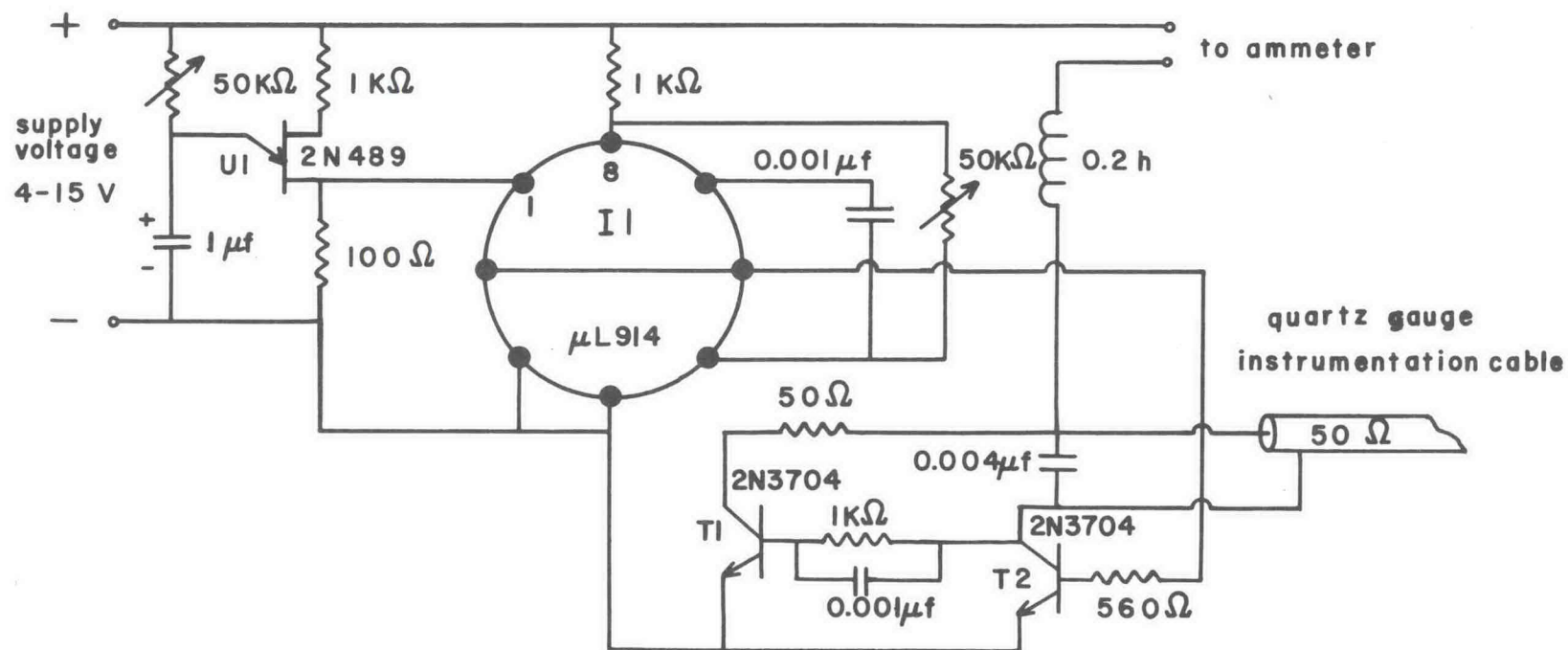
Fig. 20. Diagram of quartz calibration circuit.
